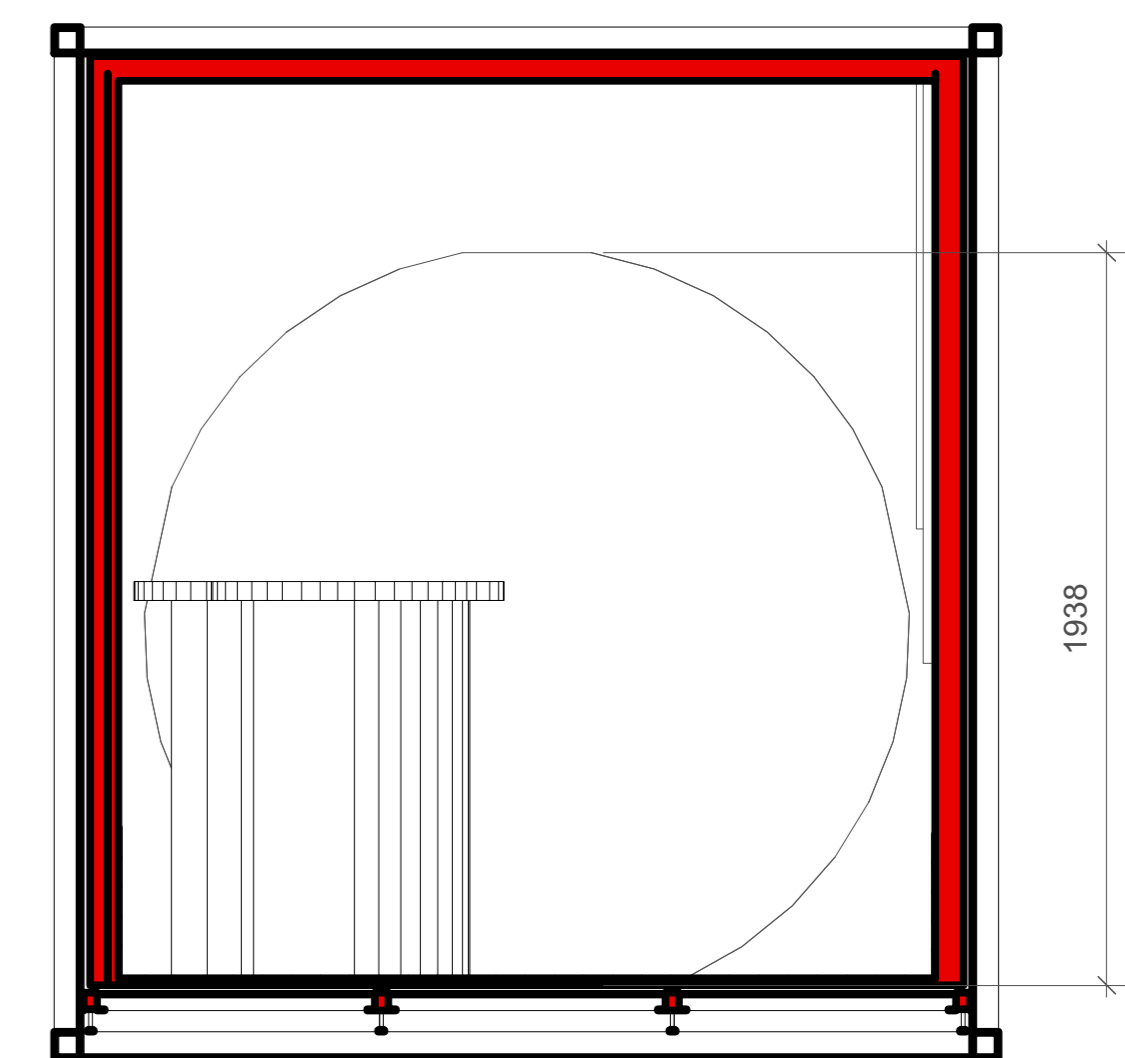
Doorsnede midden - links
